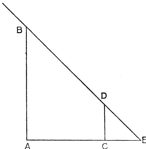
FIG. 13.—DETERMINATION OF HEIGHT OF A TREE.
